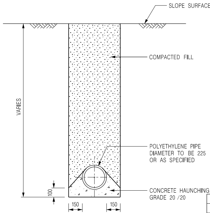
TYPICAL SECTION OF DRAIN FROM MANHOLE
