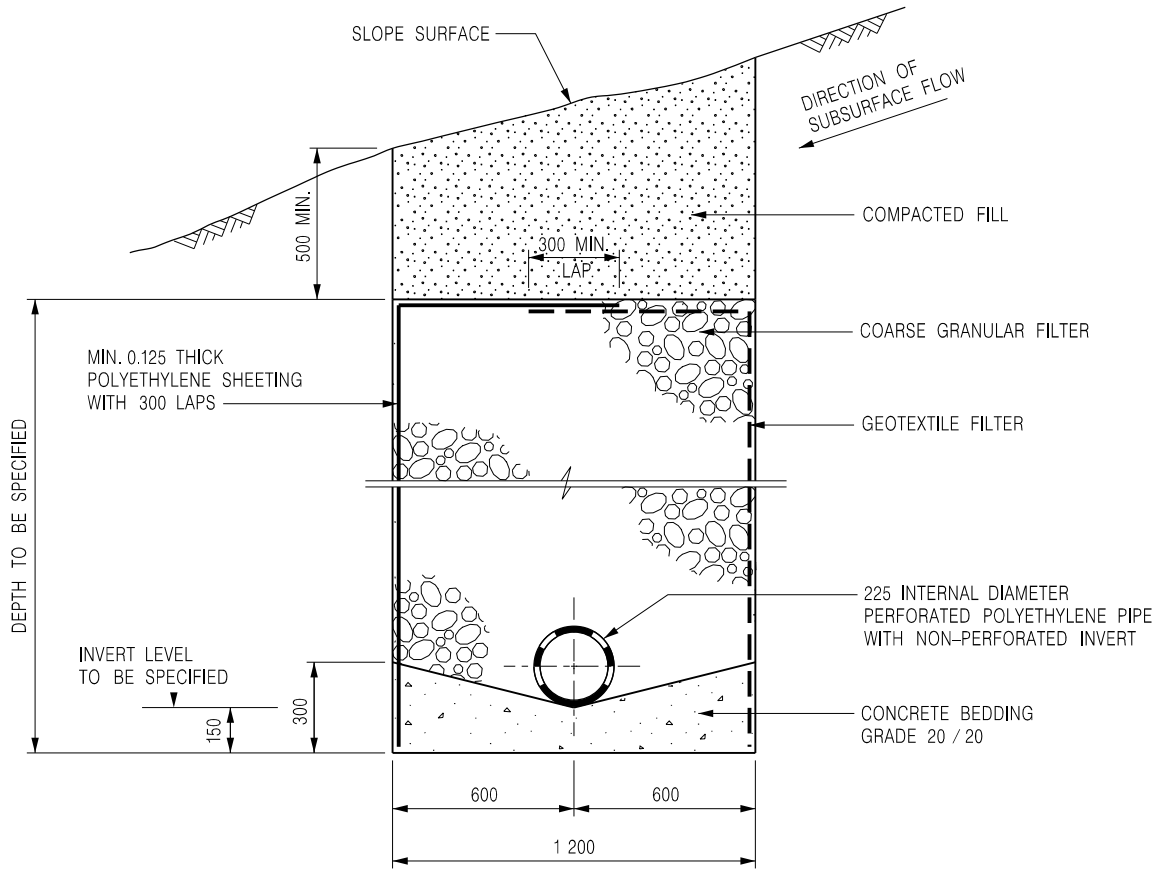
TYPICAL SECTION OF CUT-OFF DRAIN
